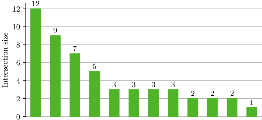
Expansion Intersections (pass@256 Base=0, RL=1), Model: EuroLLM-9B-Instruct
